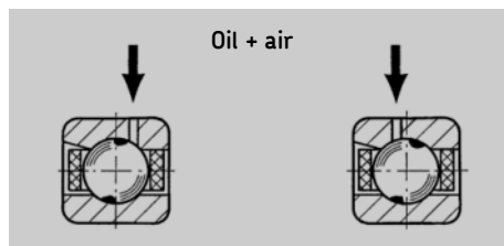
Figure 6: Lubricant delivery through outer ring
