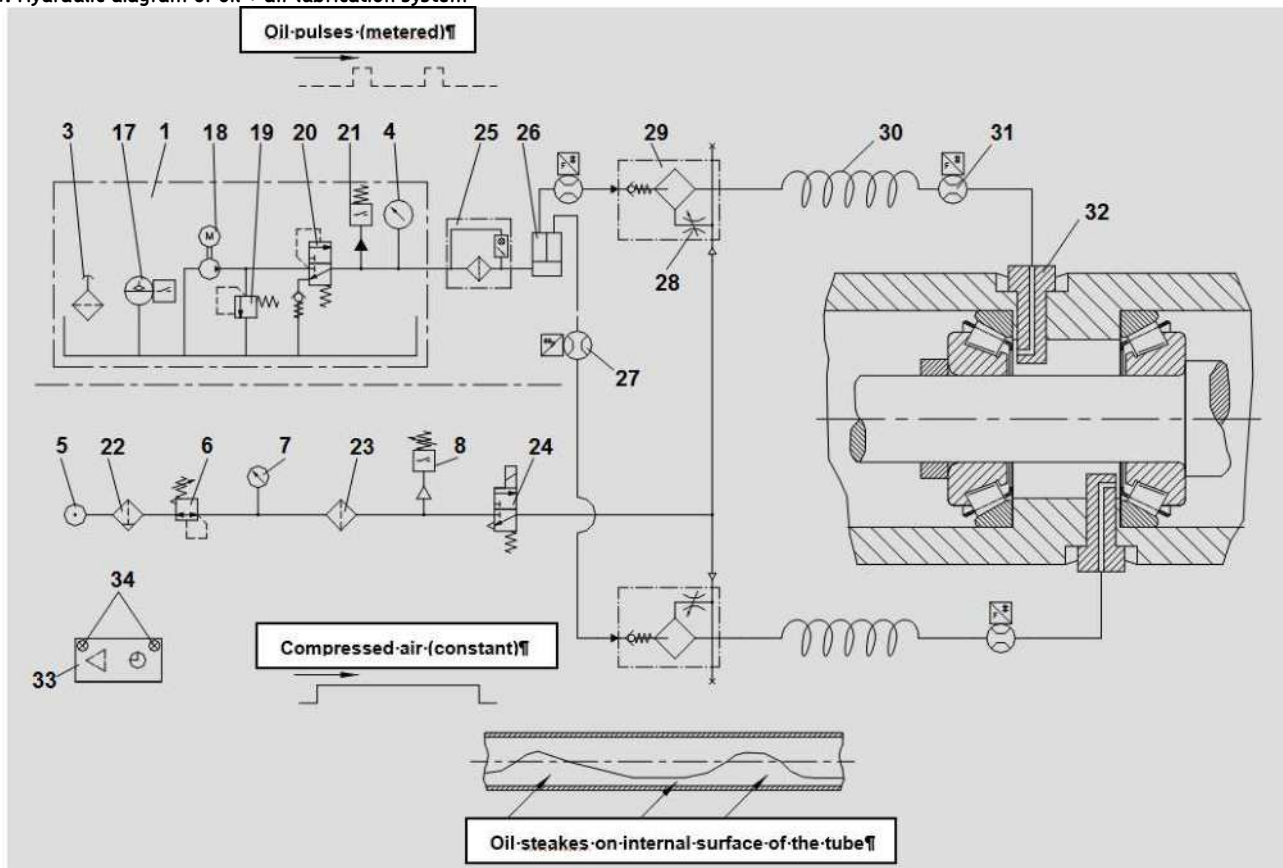
Figure 4: Hydraulic diagram of oil + air lubrication system
