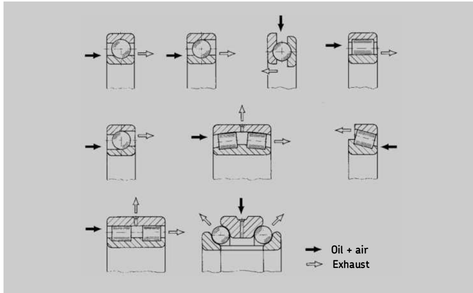
Figure 7: Lubricant delivery on various types of ball bearings
