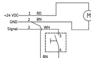
Circuit diagram of low-level signal
