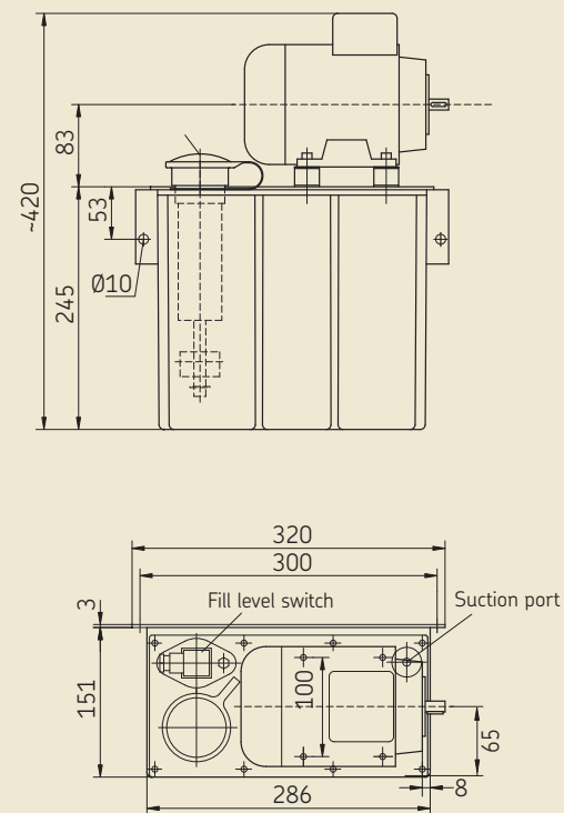
RA, electric motor drive, with 7-liter oil reservoir
