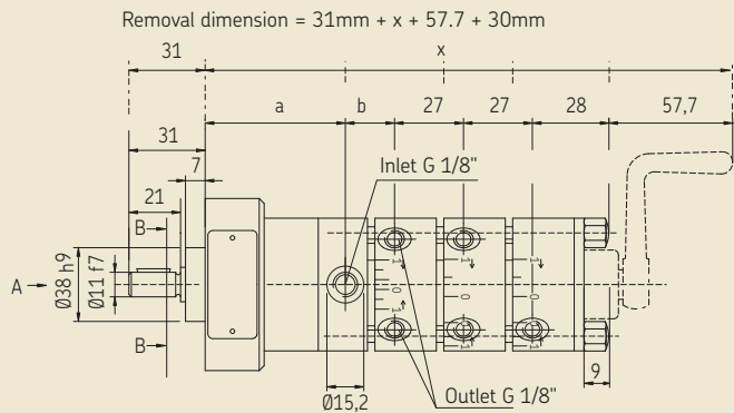
RA, rotary drive with coaxial gear
