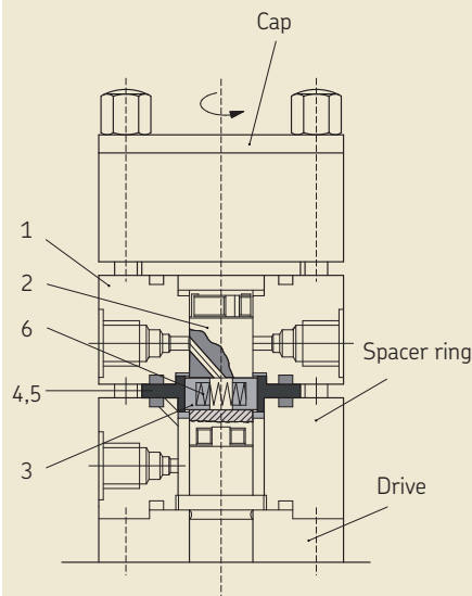
Fig. 1 Pump element in the pressure phase
