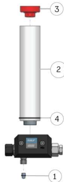
Lube-shuttle grease cartridge (363069)
