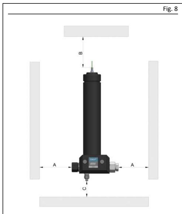
Assembly dimensions (362945)
